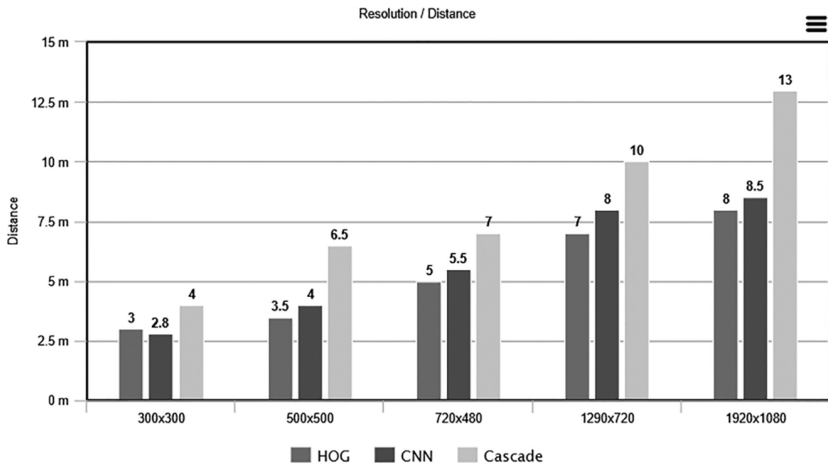
Fig. 8 Input video resolution / maximum face distance from the camera relationship for the HOG, CNN and the Haar Cascade algorithms
